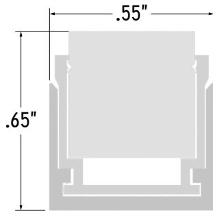
Assembled End View
