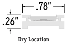
Assembled End View
