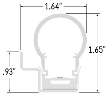
Assembled End View
