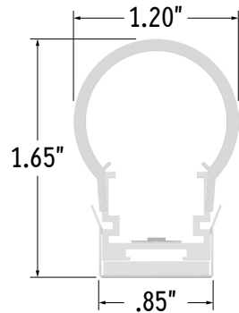
Assembled End View
