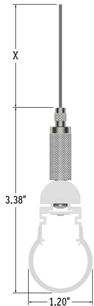
Assembled End View
