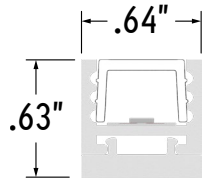
Assembled End View
