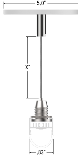
Pendant Mount (Pictured with Canopy) (LLED8000-SRT-PM-X) (X = Specify Length)
