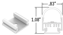
Surface Mounting Clip (LLED8000-SRT-MC)
