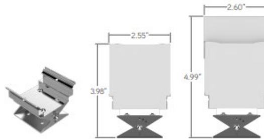
Mounting Clip (Adjustable with Locking Mechanism) (ALS600T-MC-3)
