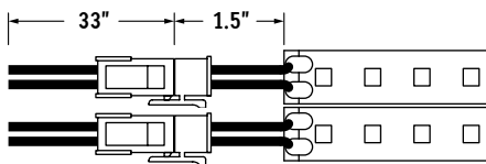
Power Connector (#LLED8000-PC-2)
