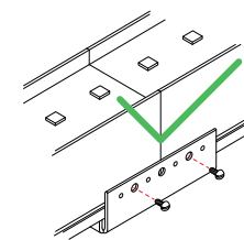
CORRECT Install outer screws on each side of mounting clip at seam
