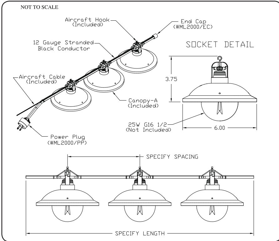
Drawing # ML2
