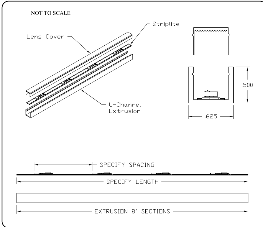
Drawing # LL5
